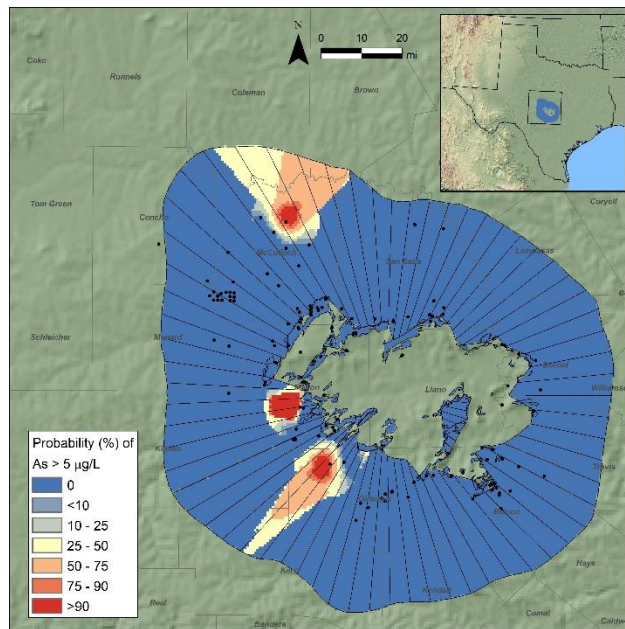
Figure 21. Hickory aquifer probability distribution of arsenic >5 µg/L. There are no groundwater samples from the Hickory aquifer that exceed the 10 µg/L MCL concentration.
