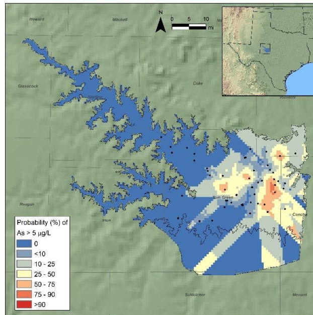
Figure 23. Lipan aquifer probability distribution of arsenic >5 µg/L. There are no groundwater samples from the Lipan aquifer that exceeded the 10 µg/L MCL concentration.
